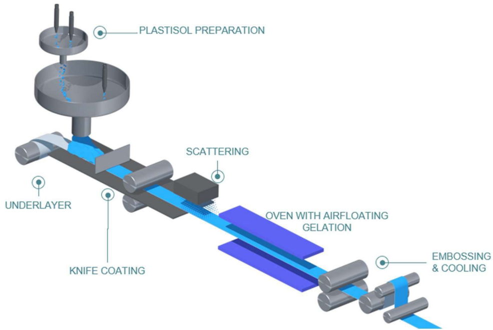
Figure 3: Coating process
